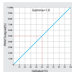
Lineare Dimmkurve
